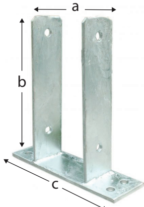
U Anchor
